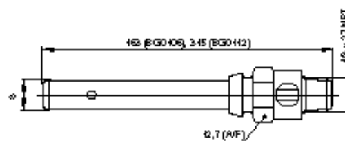
Extension tubes BG0106, BG0112
